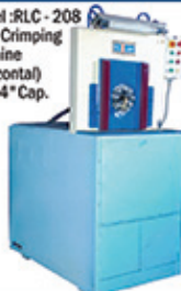
Low Pressure Motorised Hose Crimping Machine Upto 1"
